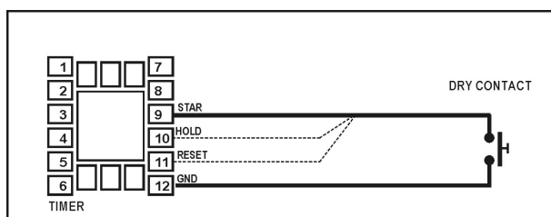
Figure 03 - Connecting dry contact (relay, switch key)
