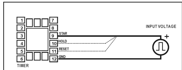
Figure 04 - Connection for pulse input.
